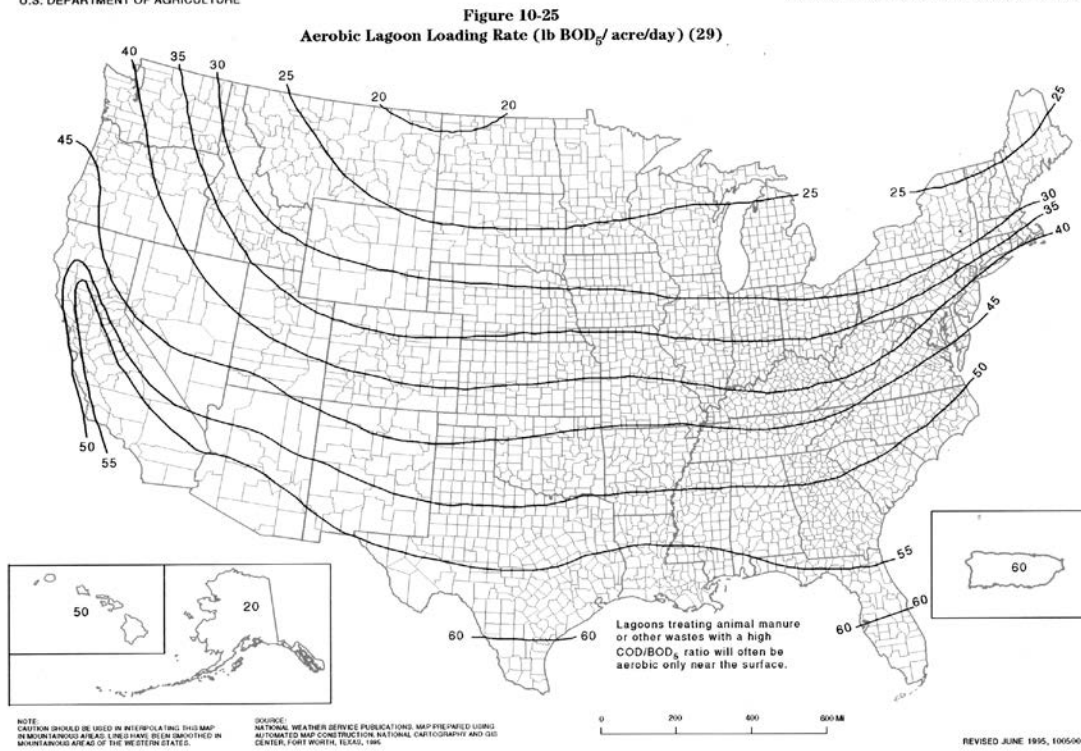
Figure 2. Aerobic lagoon loading rate
