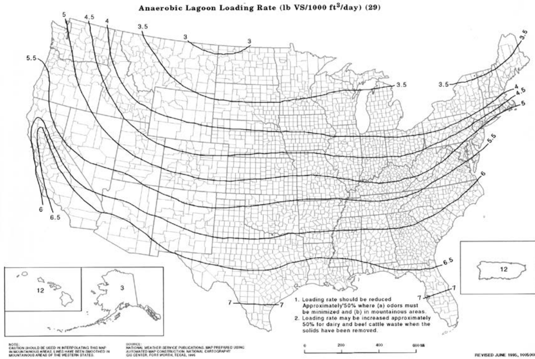
Figure 1. Anaerobic loading rate
